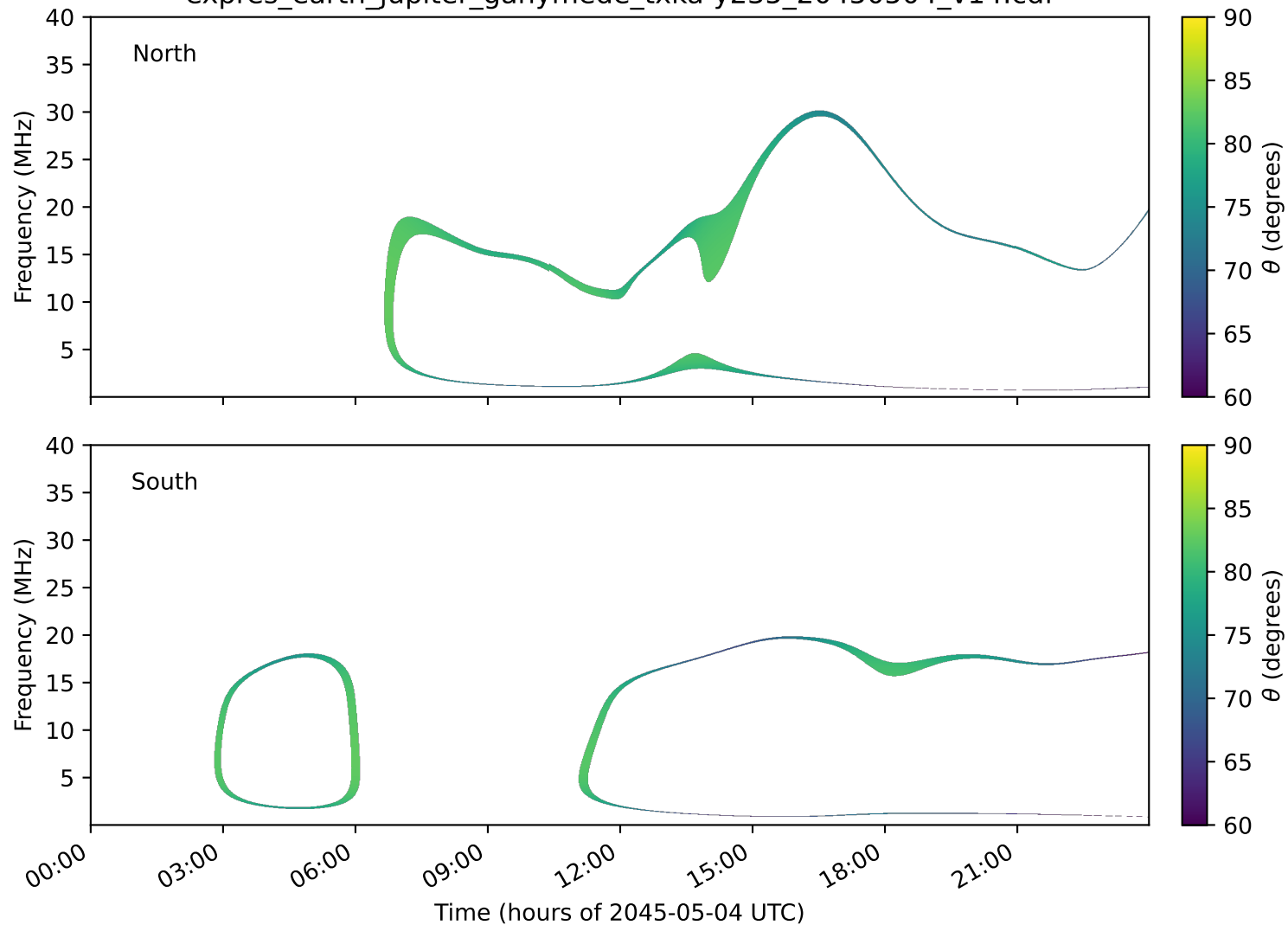
expres_earth_jupiter_ganymede_txka-y235_20450504_v14.cdf
