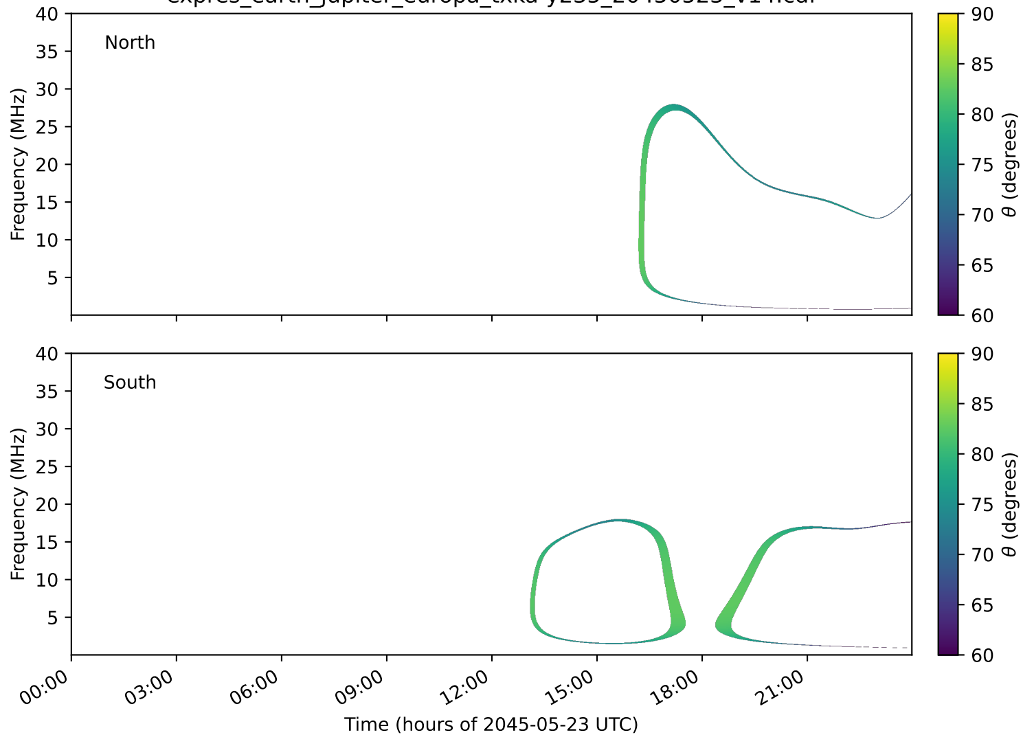
expres_earth_jupiter_europa_txka-y235_20450523_v14.cdf
