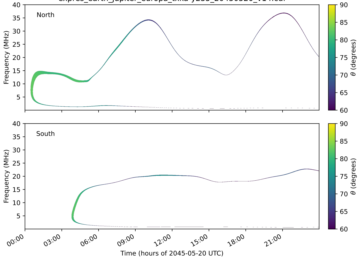
expres_earth_jupiter_europa_txka-y235_20450520_v14.cdf
