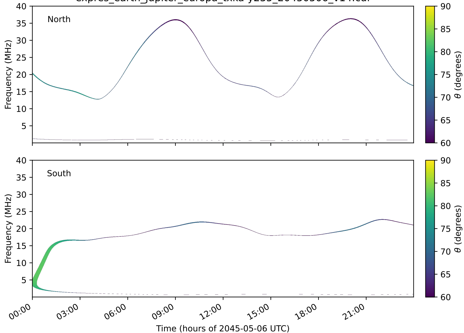
expres_earth_jupiter_europa_txka-y235_20450506_v14.cdf
