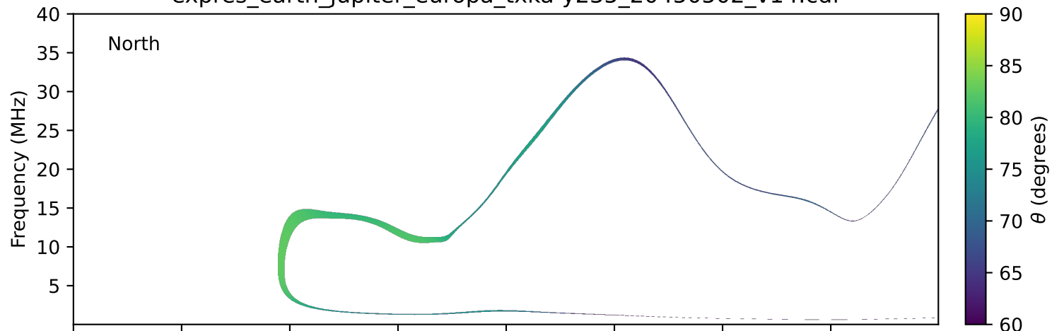
expres_earth_jupiter_europa_txka-y235_20450502_v14.cdf
