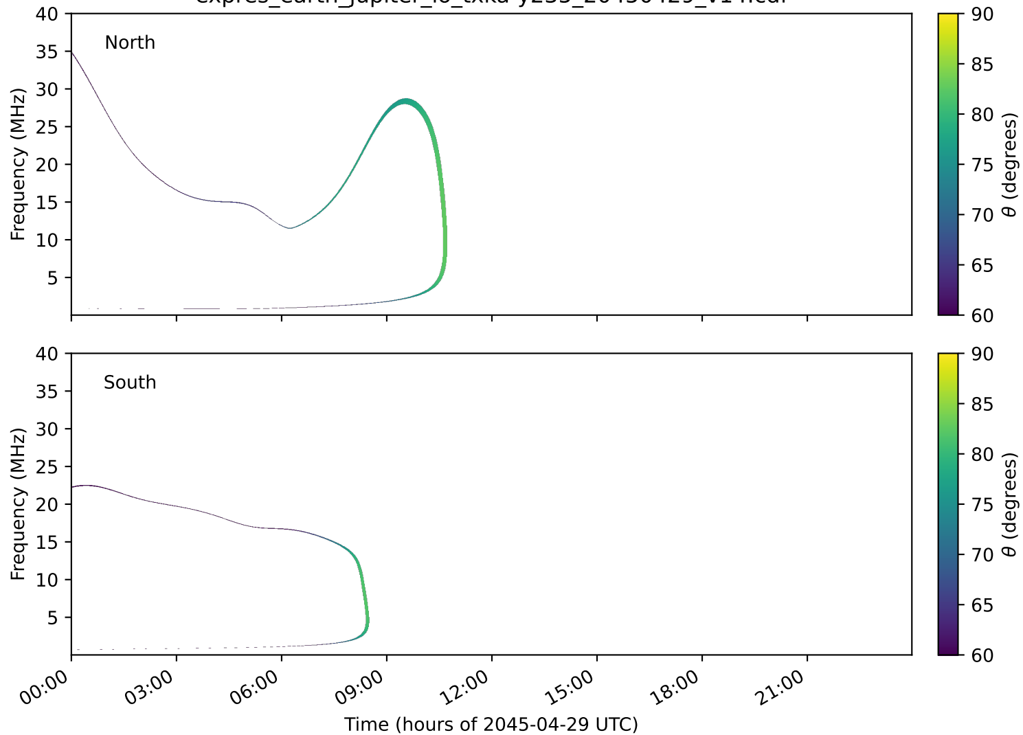
expres_earth_jupiter_io_txka-y235_20450429_v14.cdf
