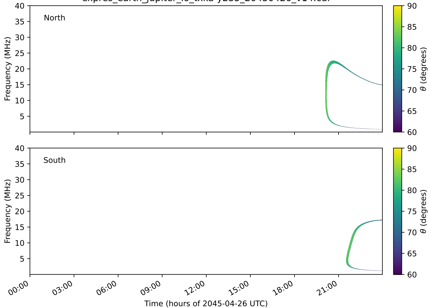
expres_earth_jupiter_io_txka-y235_20450426_v14.cdf
