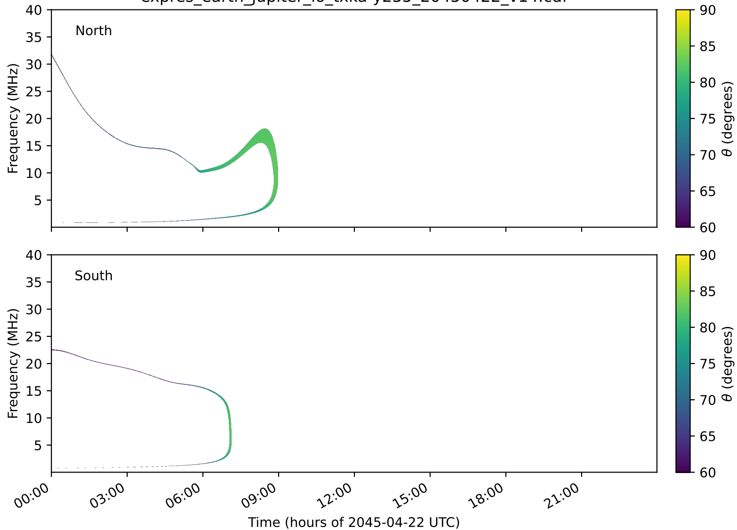
expres_earth_jupiter_io_txka-y235_20450422_v14.cdf
