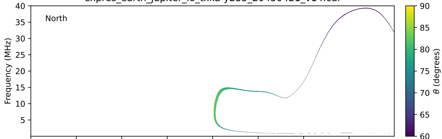
expres_earth_jupiter_io_txka-y235_20450421_v14.cdf
