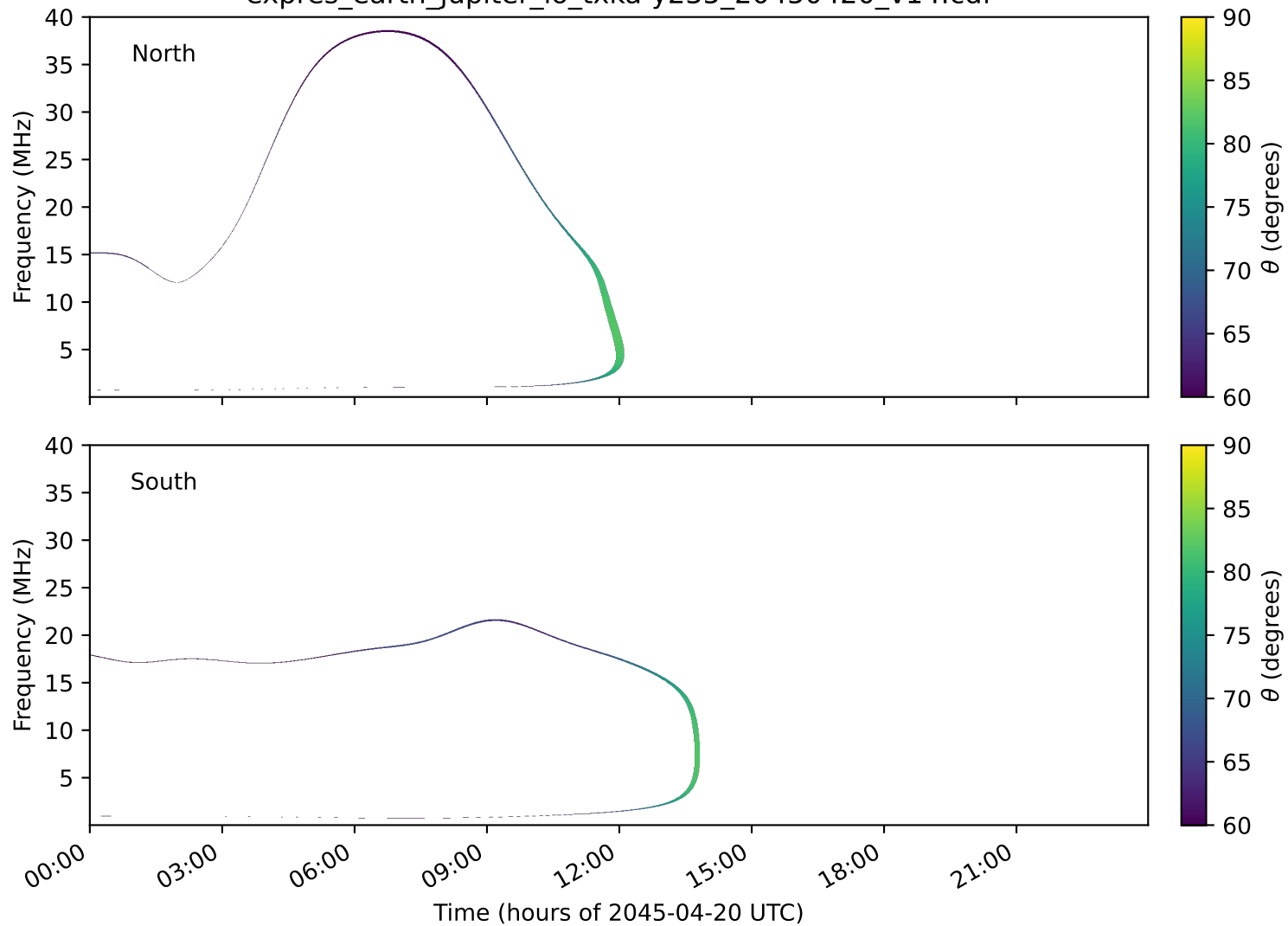
expres_earth_jupiter_io_txka-y235_20450420_v14.cdf
