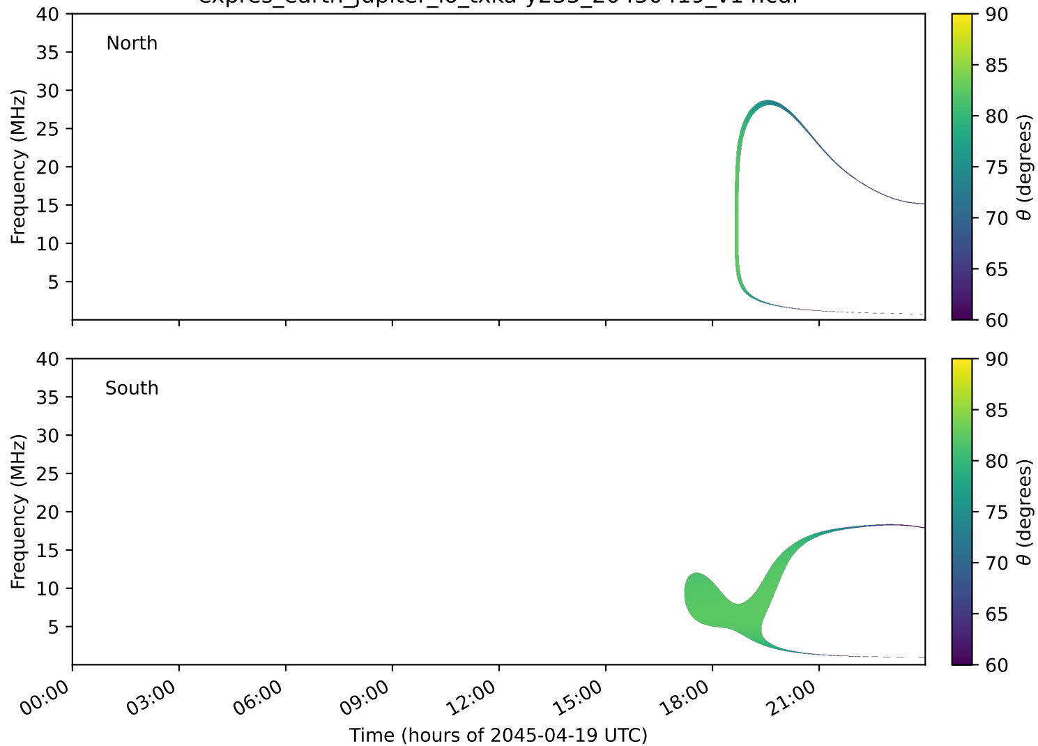
expres_earth_jupiter_io_txka-y235_20450419_v14.cdf
