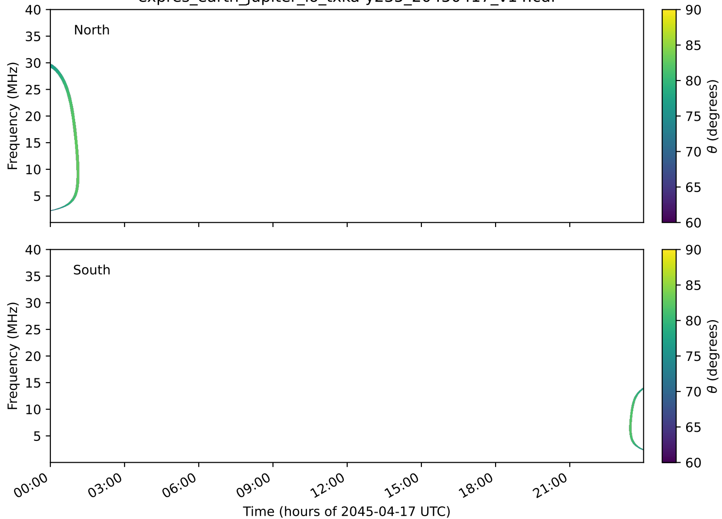
expres_earth_jupiter_io_txka-y235_20450417_v14.cdf
