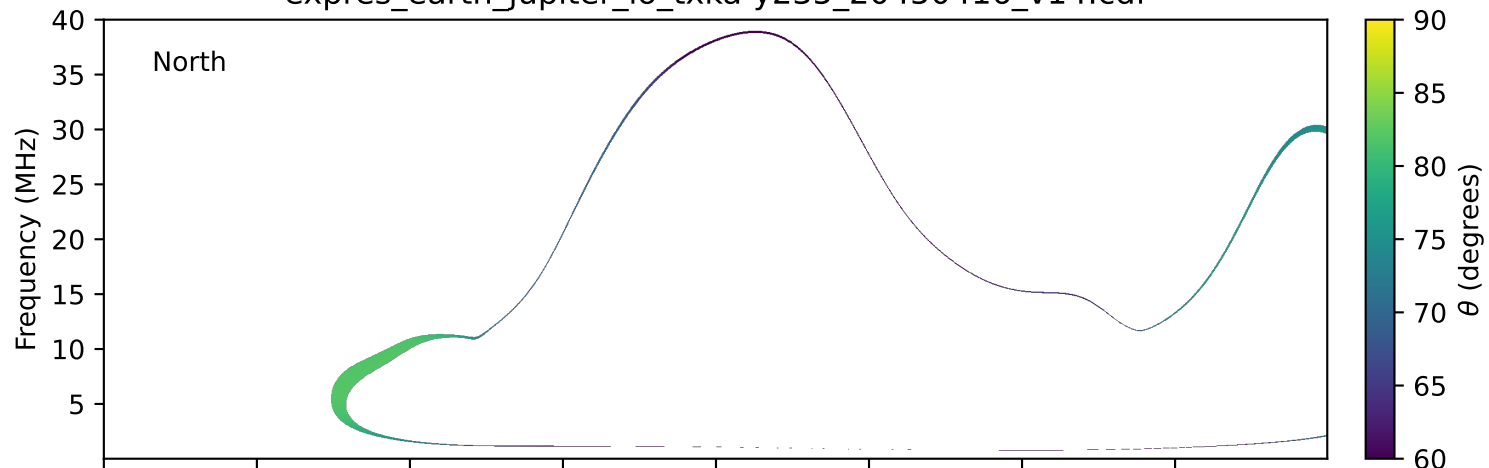
expres_earth_jupiter_io_txka-y235_20450416_v14.cdf
