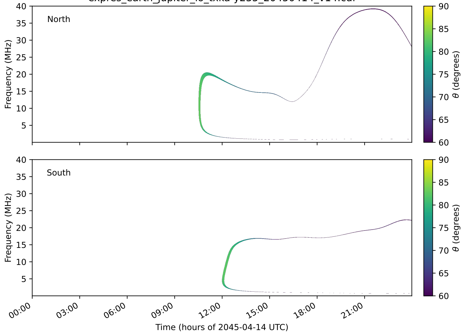
expres_earth_jupiter_io_txka-y235_20450414_v14.cdf
