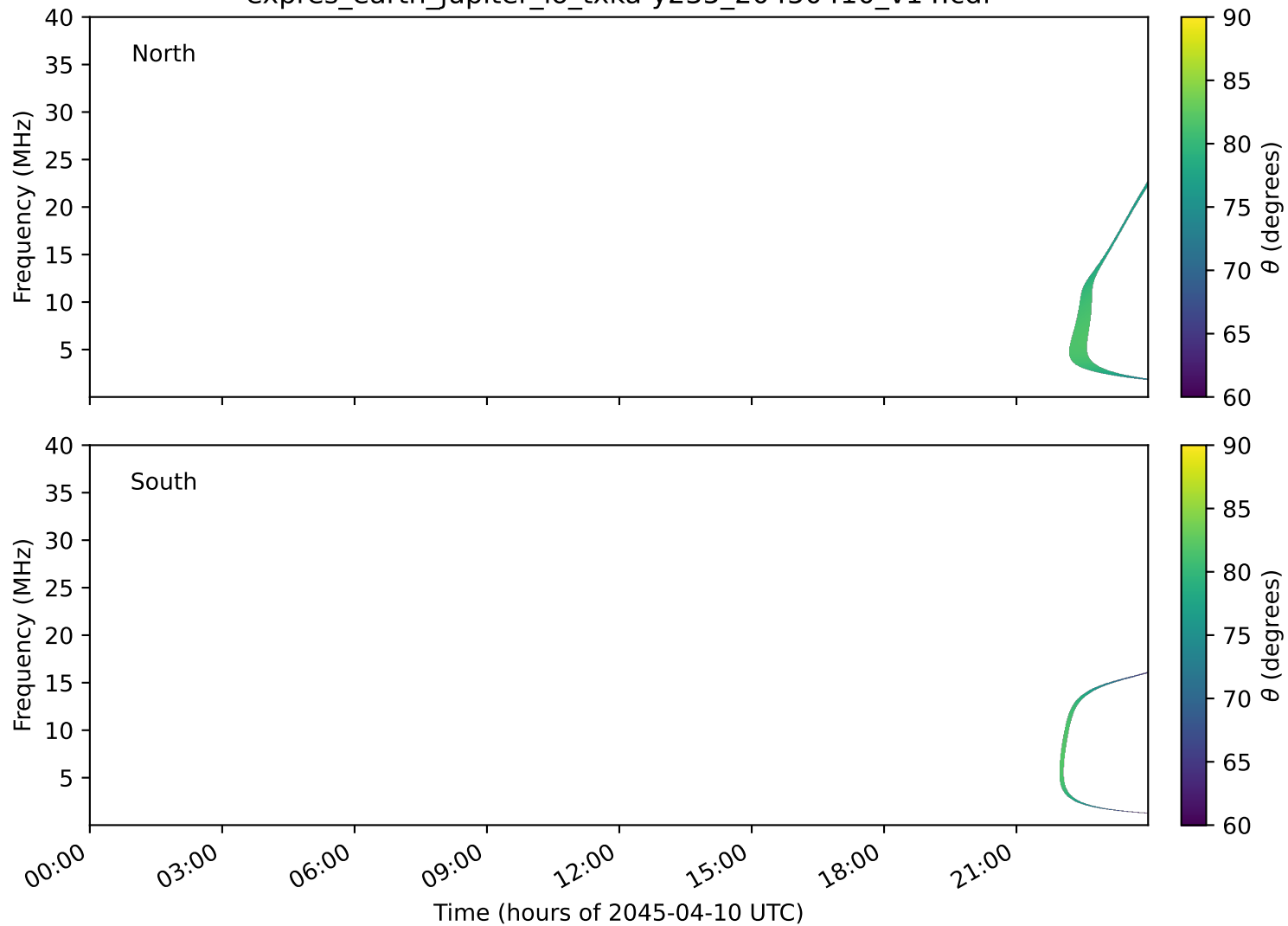
expres_earth_jupiter_io_txka-y235_20450410_v14.cdf
