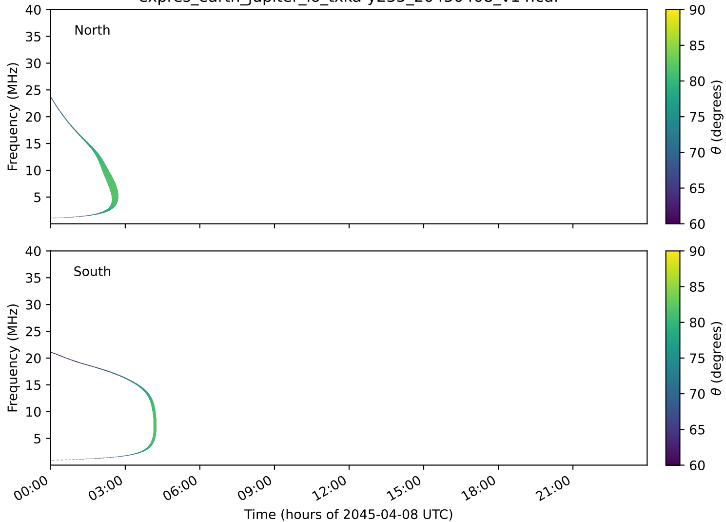
expres_earth_jupiter_io_txka-y235_20450408_v14.cdf
