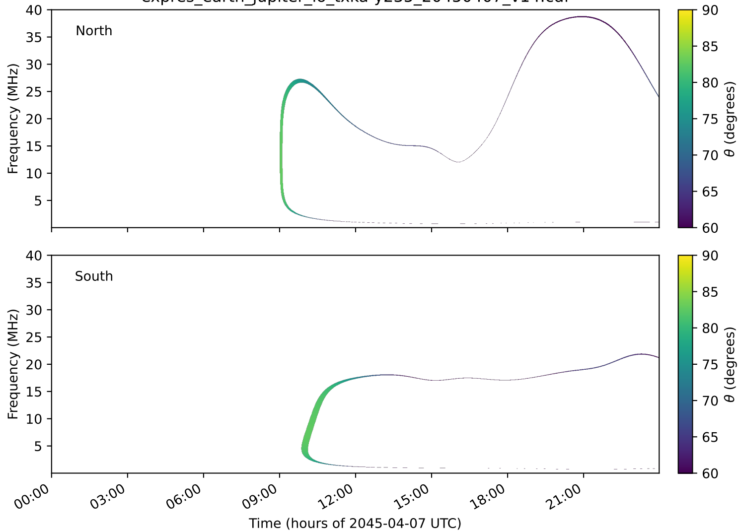
expres_earth_jupiter_io_txka-y235_20450407_v14.cdf
