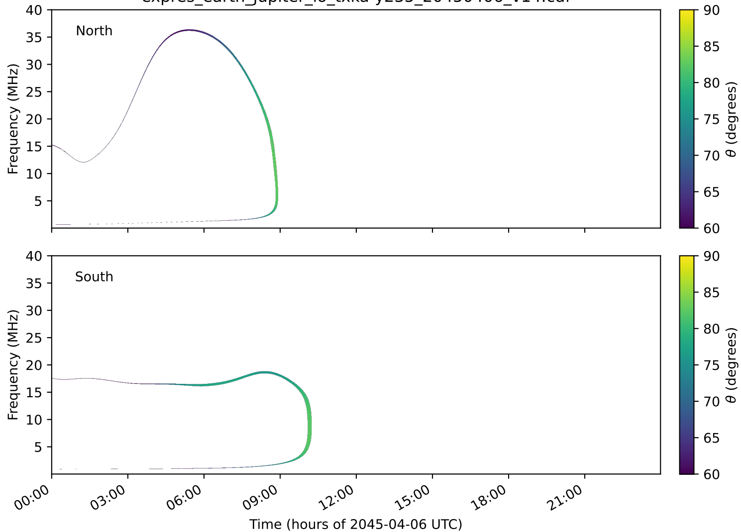
expres_earth_jupiter_io_txka-y235_20450406_v14.cdf
