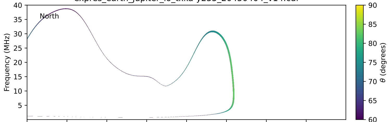
expres_earth_jupiter_io_txka-y235_20450404_v14.cdf
