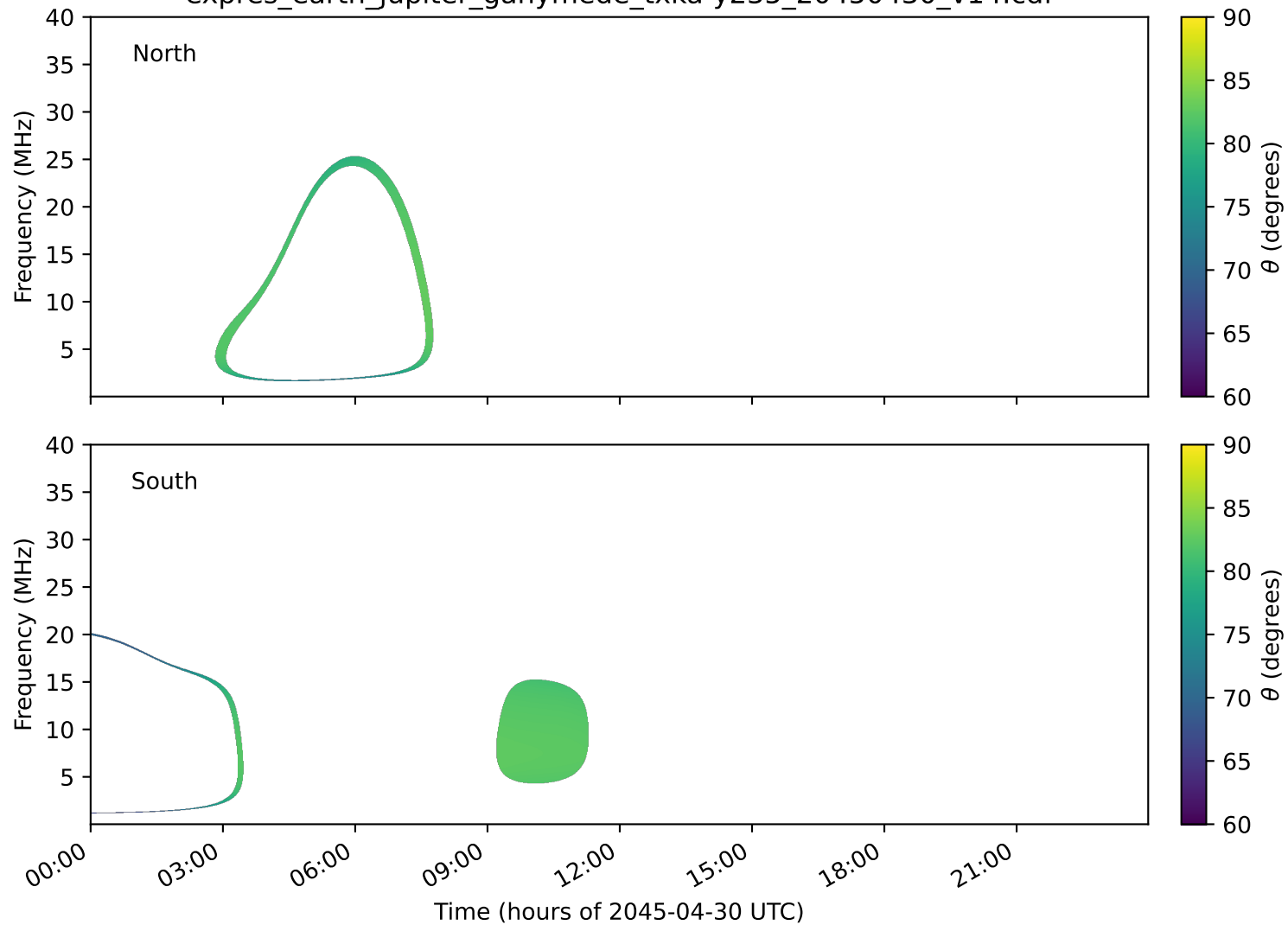
expres_earth_jupiter_ganymede_txka-y235_20450430_v14.cdf
