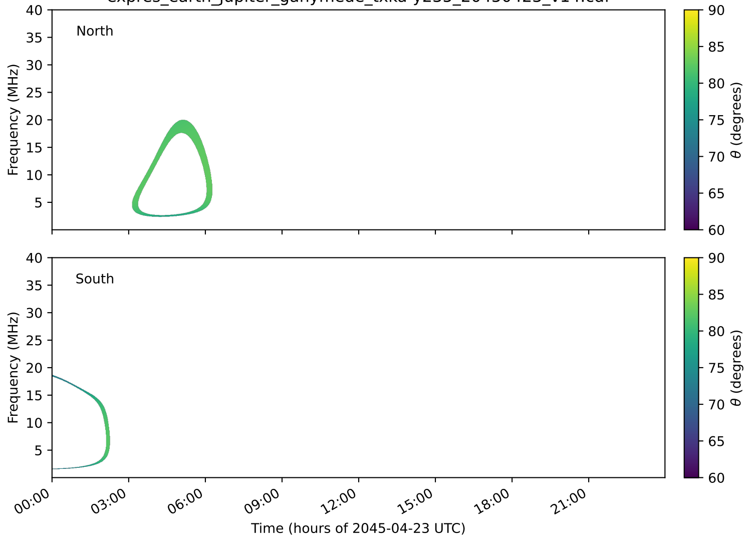
expres_earth_jupiter_ganymede_txka-y235_20450423_v14.cdf
