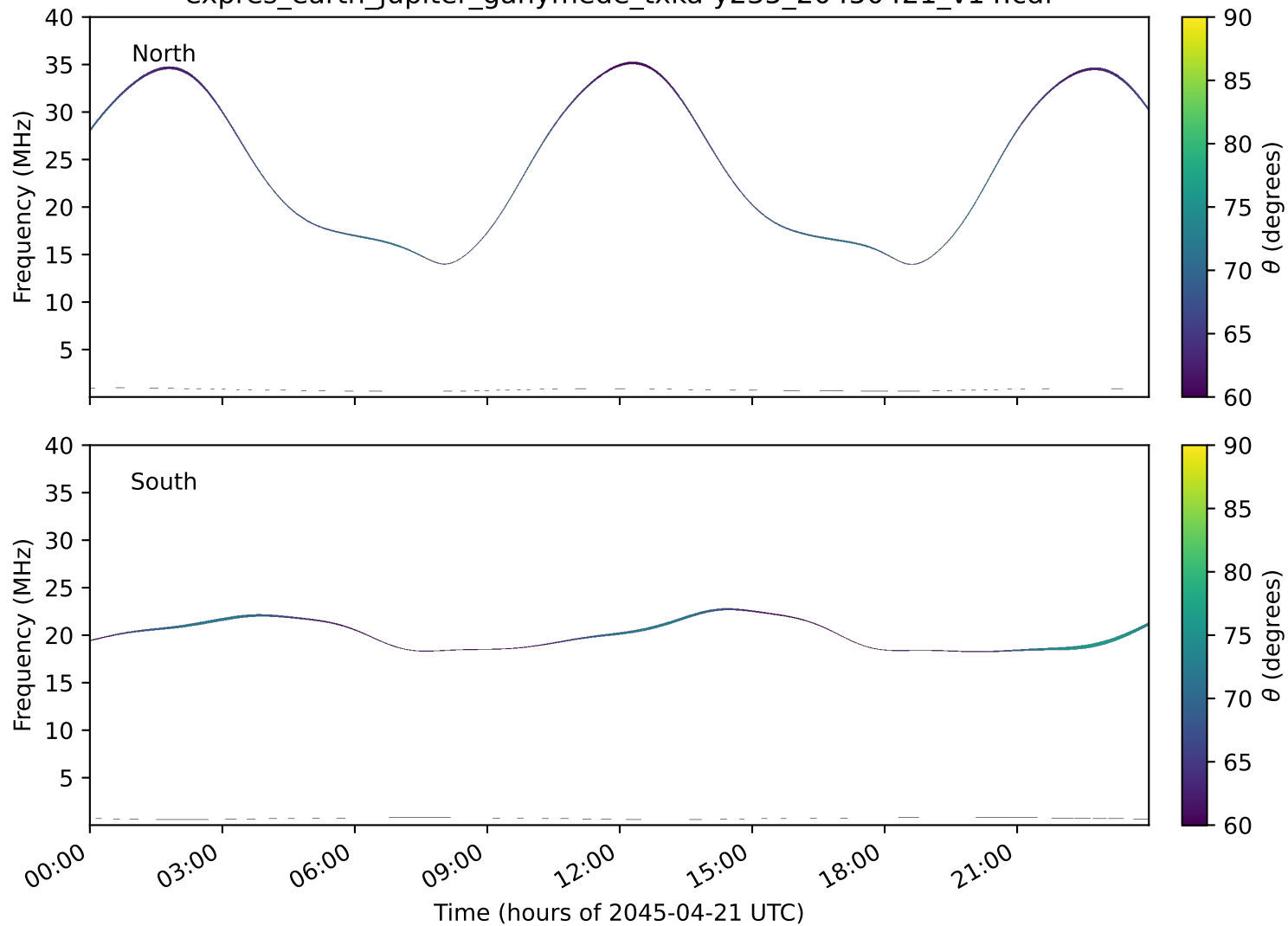
expres_earth_jupiter_ganymede_txka-y235_20450421_v14.cdf
