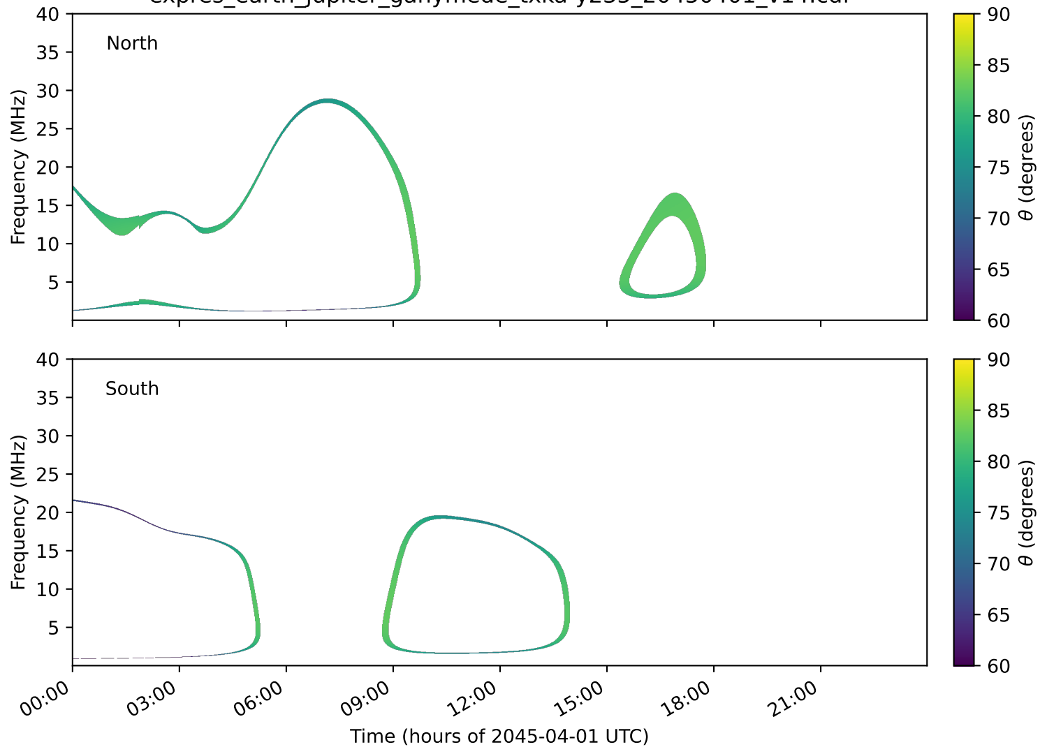
expres_earth_jupiter_ganymede_txka-y235_20450401_v14.cdf
