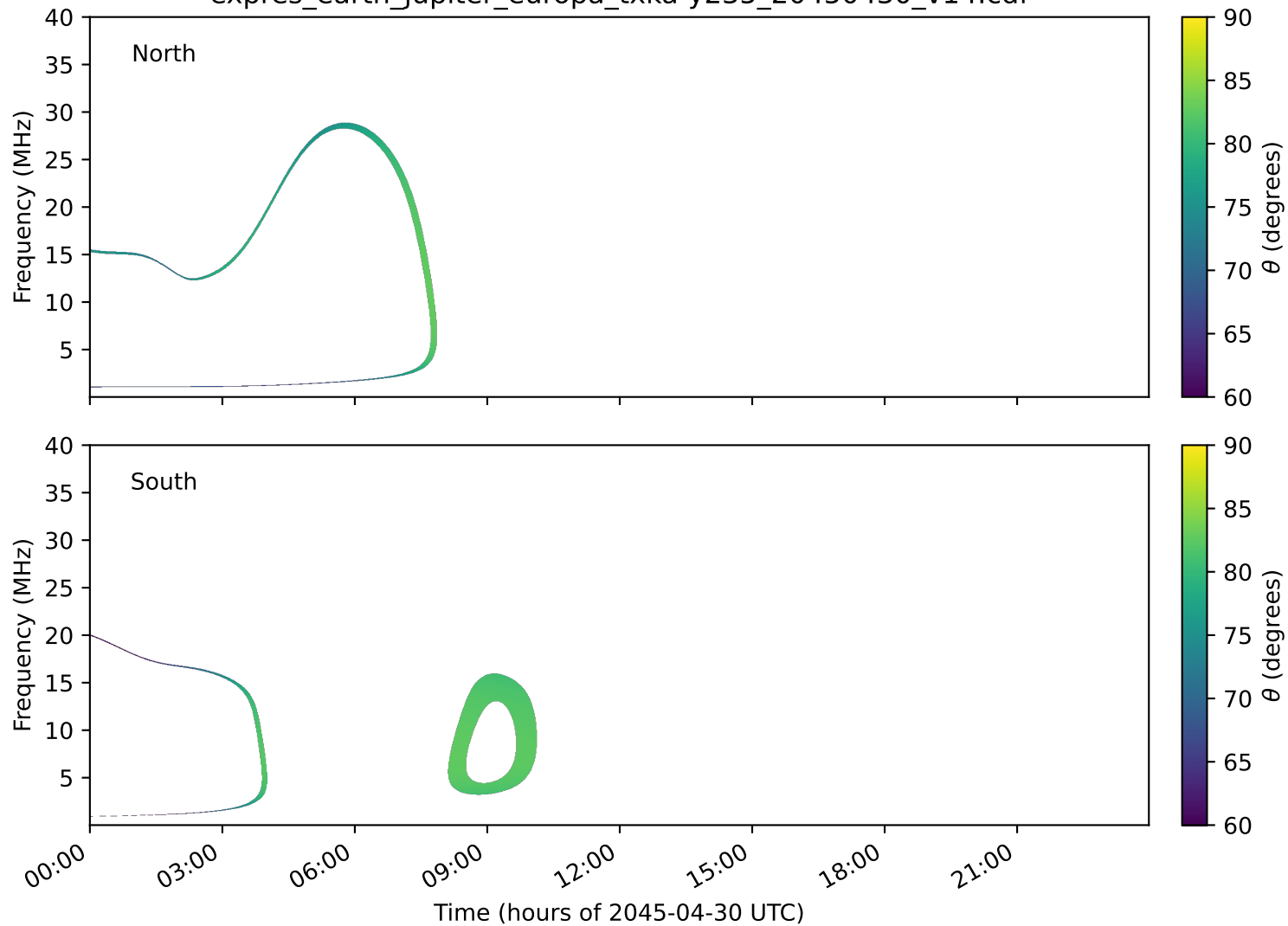
expres_earth_jupiter_europa_txka-y235_20450430_v14.cdf
