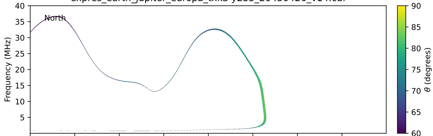
expres_earth_jupiter_europa_txka-y235_20450426_v14.cdf
