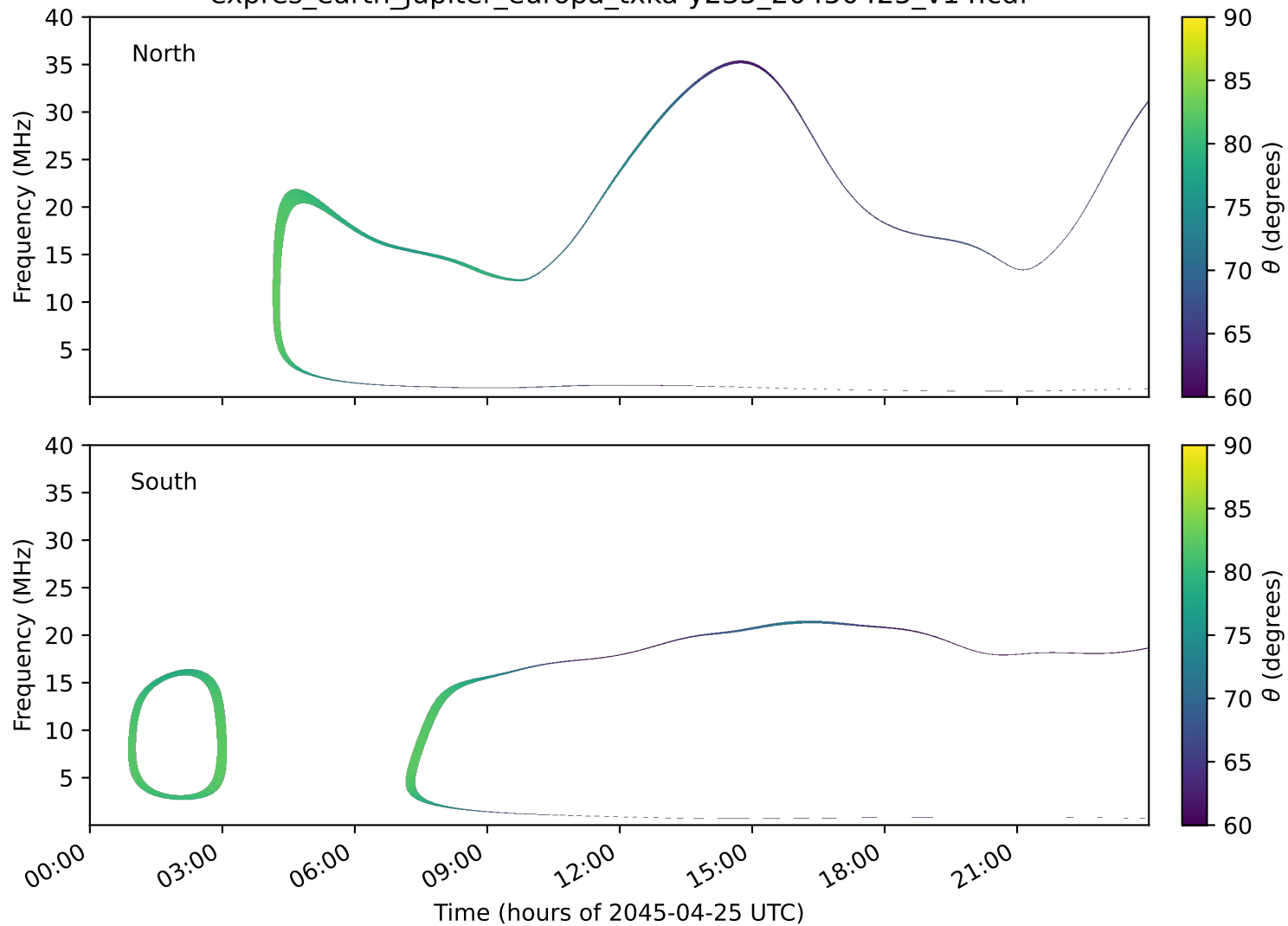
expres_earth_jupiter_europa_txka-y235_20450425_v14.cdf
