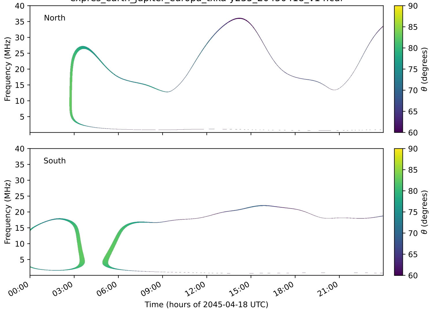
expres_earth_jupiter_europa_txka-y235_20450418_v14.cdf
