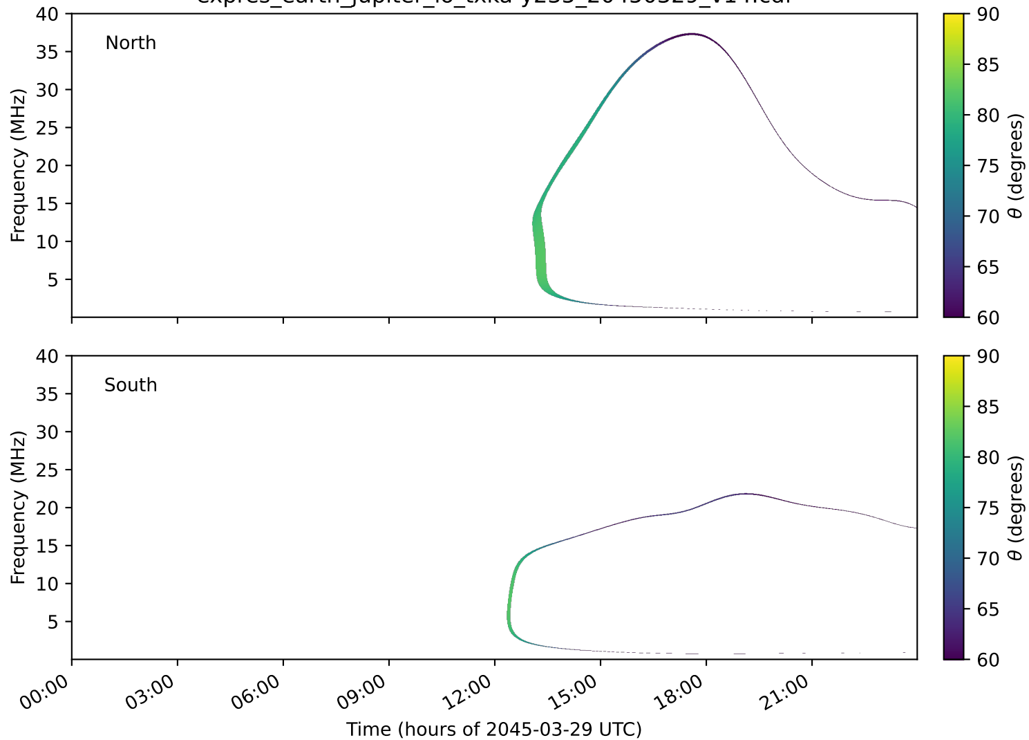
expres_earth_jupiter_io_txka-y235_20450329_v14.cdf
