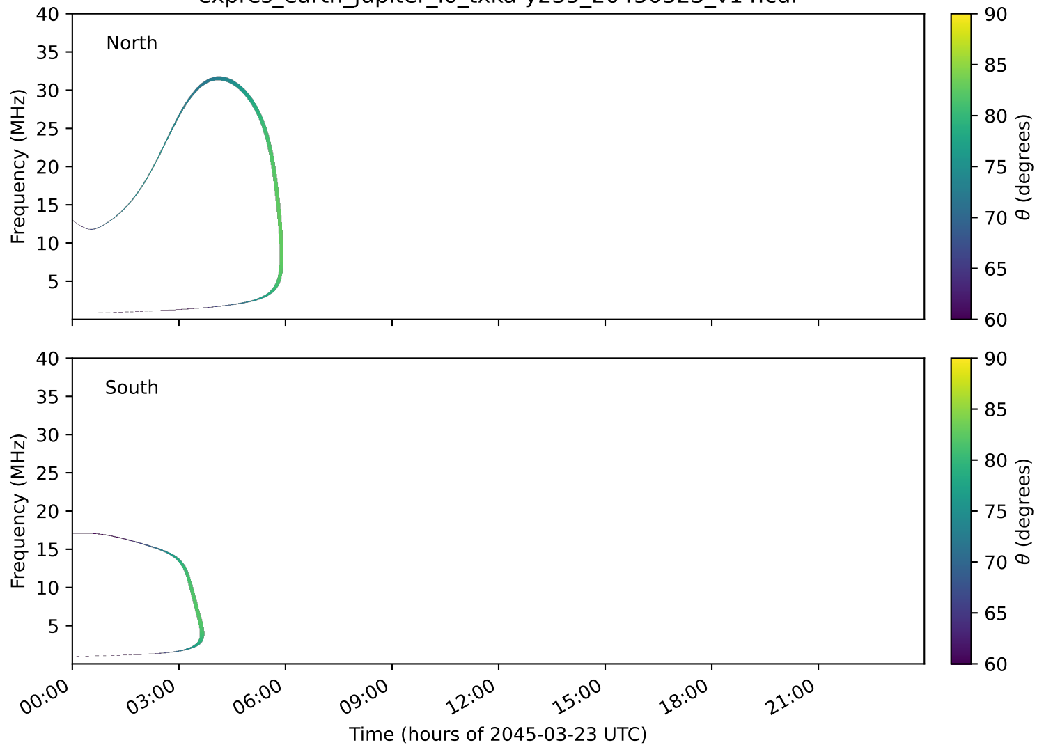
expres_earth_jupiter_io_txka-y235_20450323_v14.cdf
