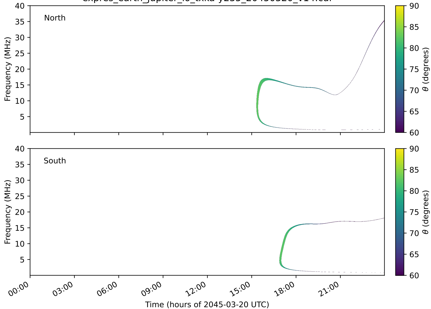
expres_earth_jupiter_io_txka-y235_20450320_v14.cdf
