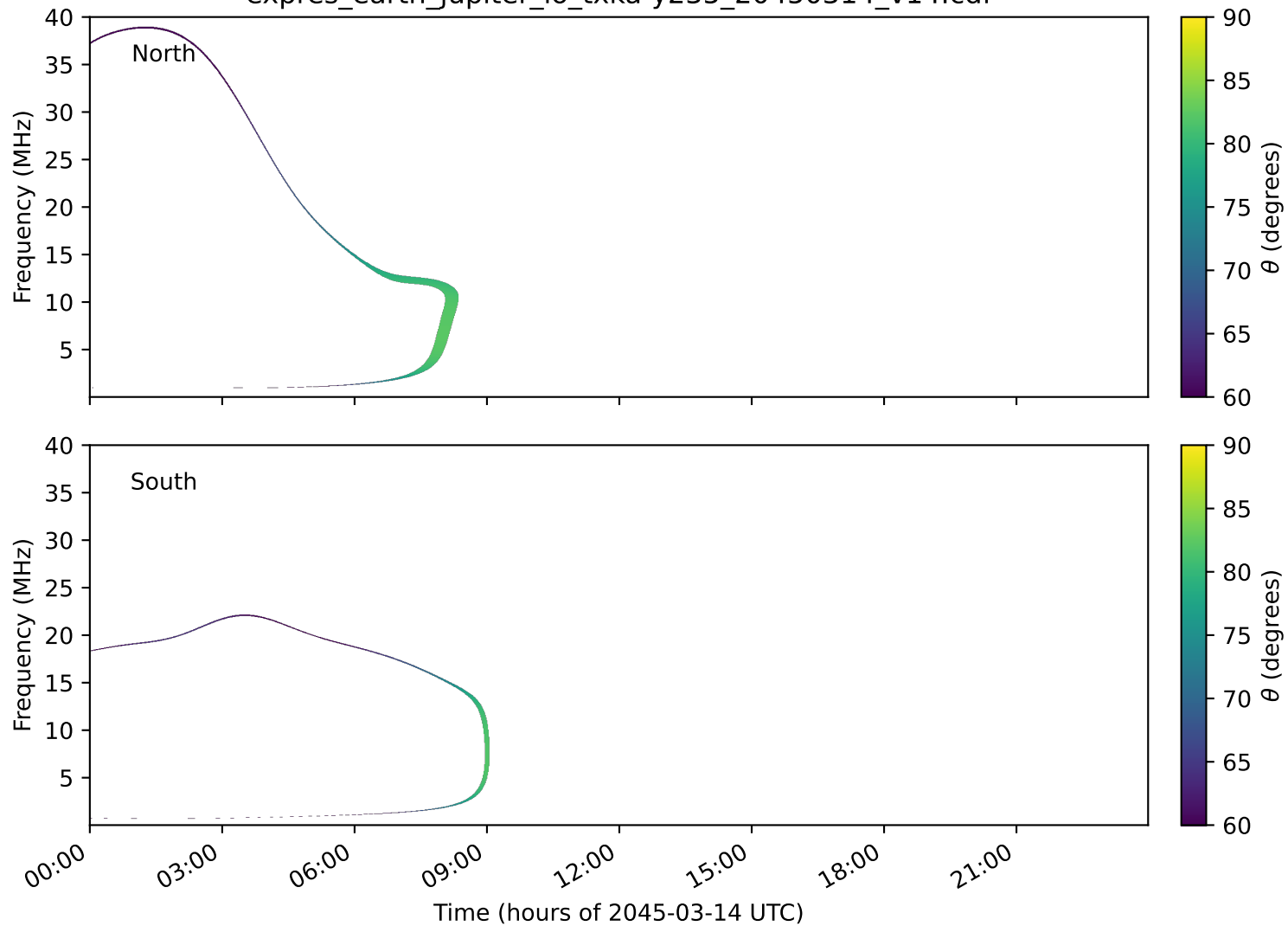
expres_earth_jupiter_io_txka-y235_20450314_v14.cdf
