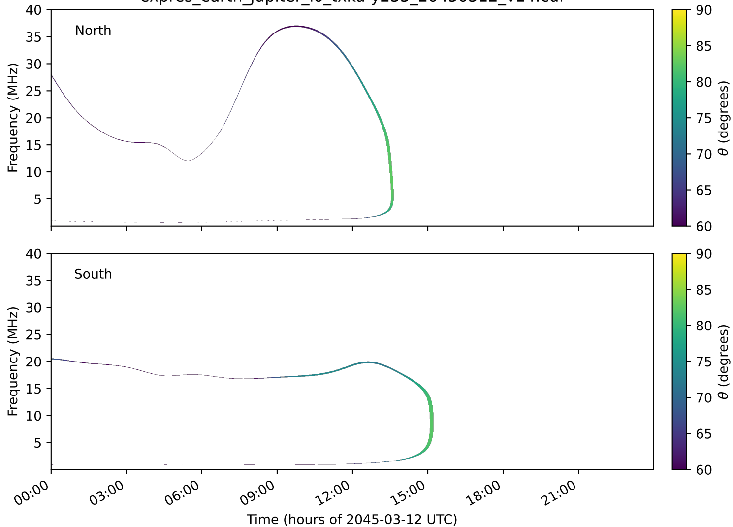
expres_earth_jupiter_io_txka-y235_20450312_v14.cdf
