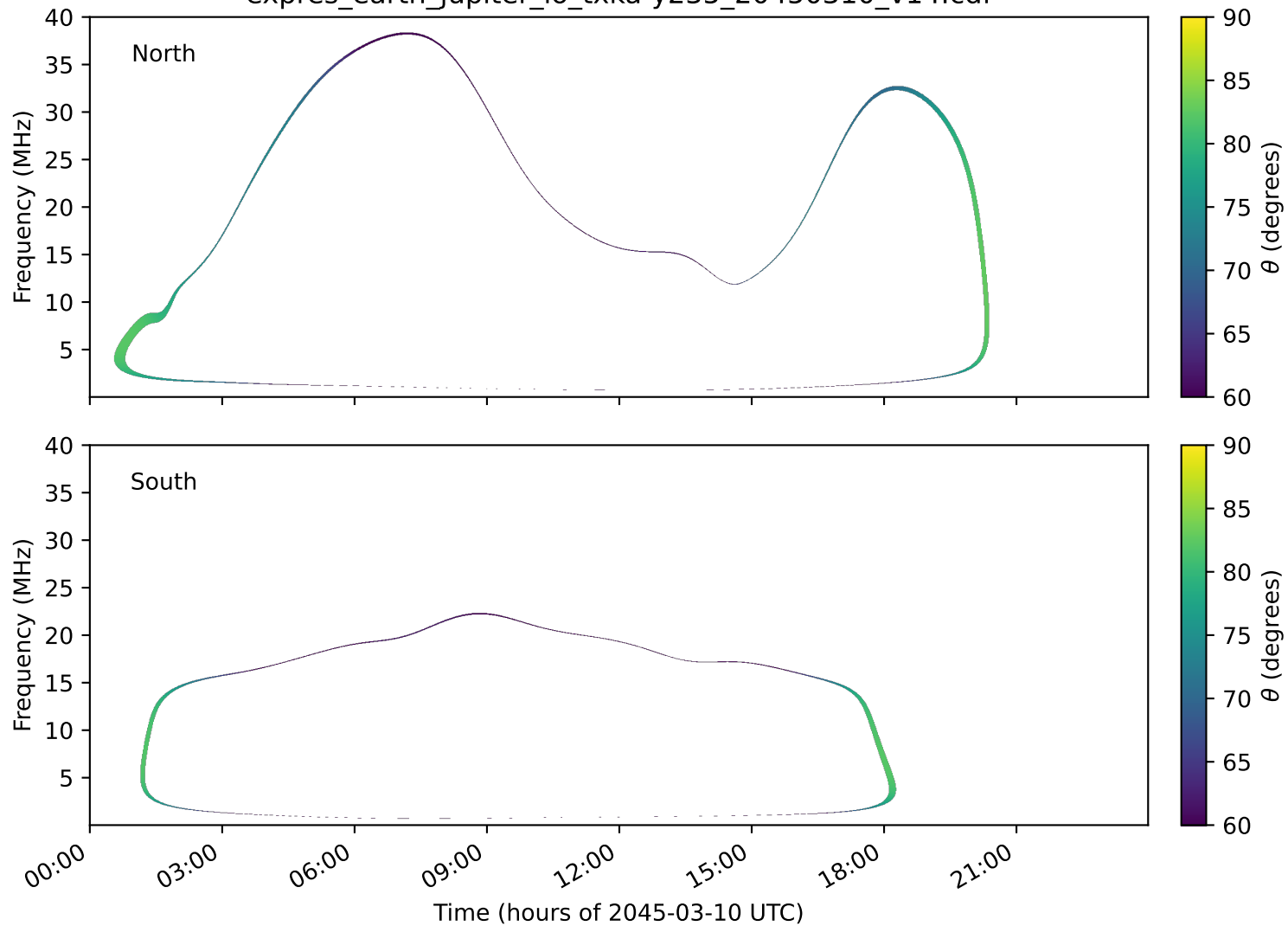
expres_earth_jupiter_io_txka-y235_20450310_v14.cdf
