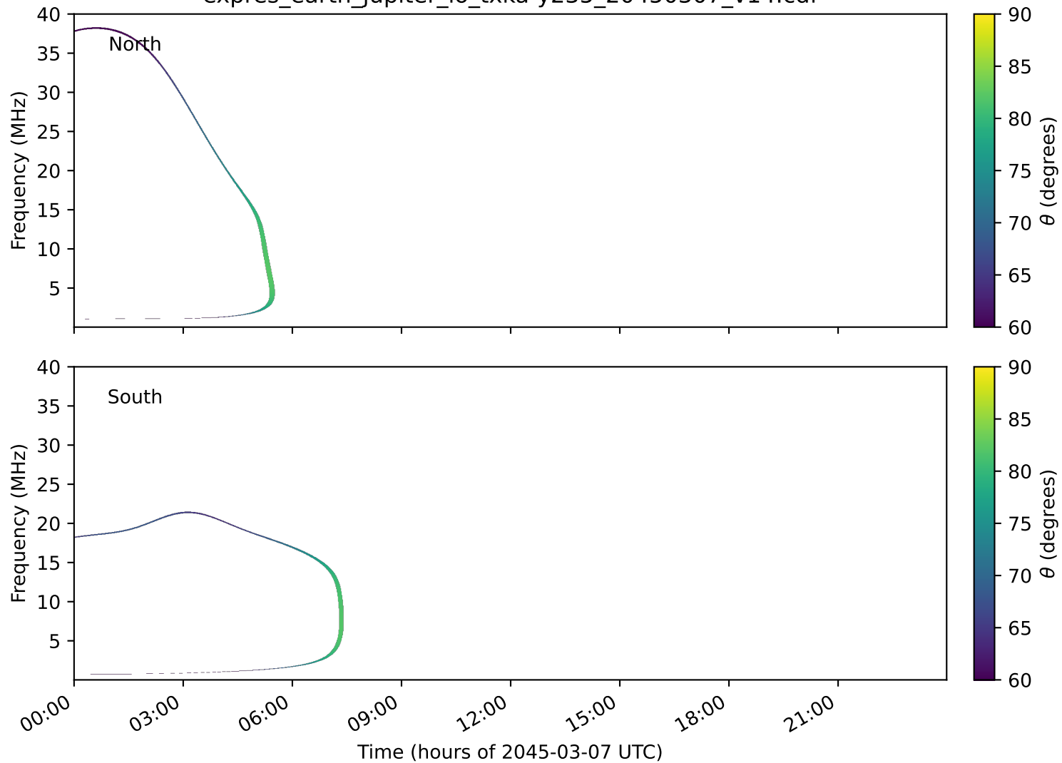
expres_earth_jupiter_io_txka-y235_20450307_v14.cdf
