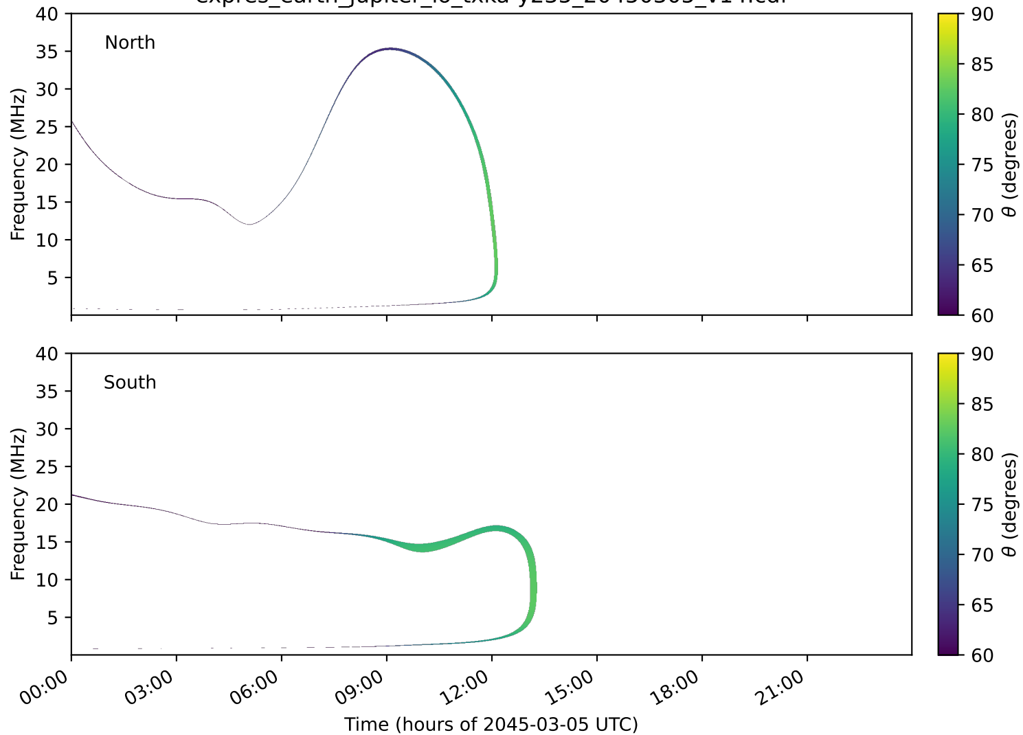
expres_earth_jupiter_io_txka-y235_20450305_v14.cdf
