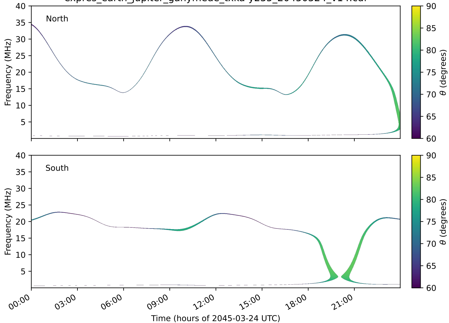
expres_earth_jupiter_ganymede_txka-y235_20450324_v14.cdf
