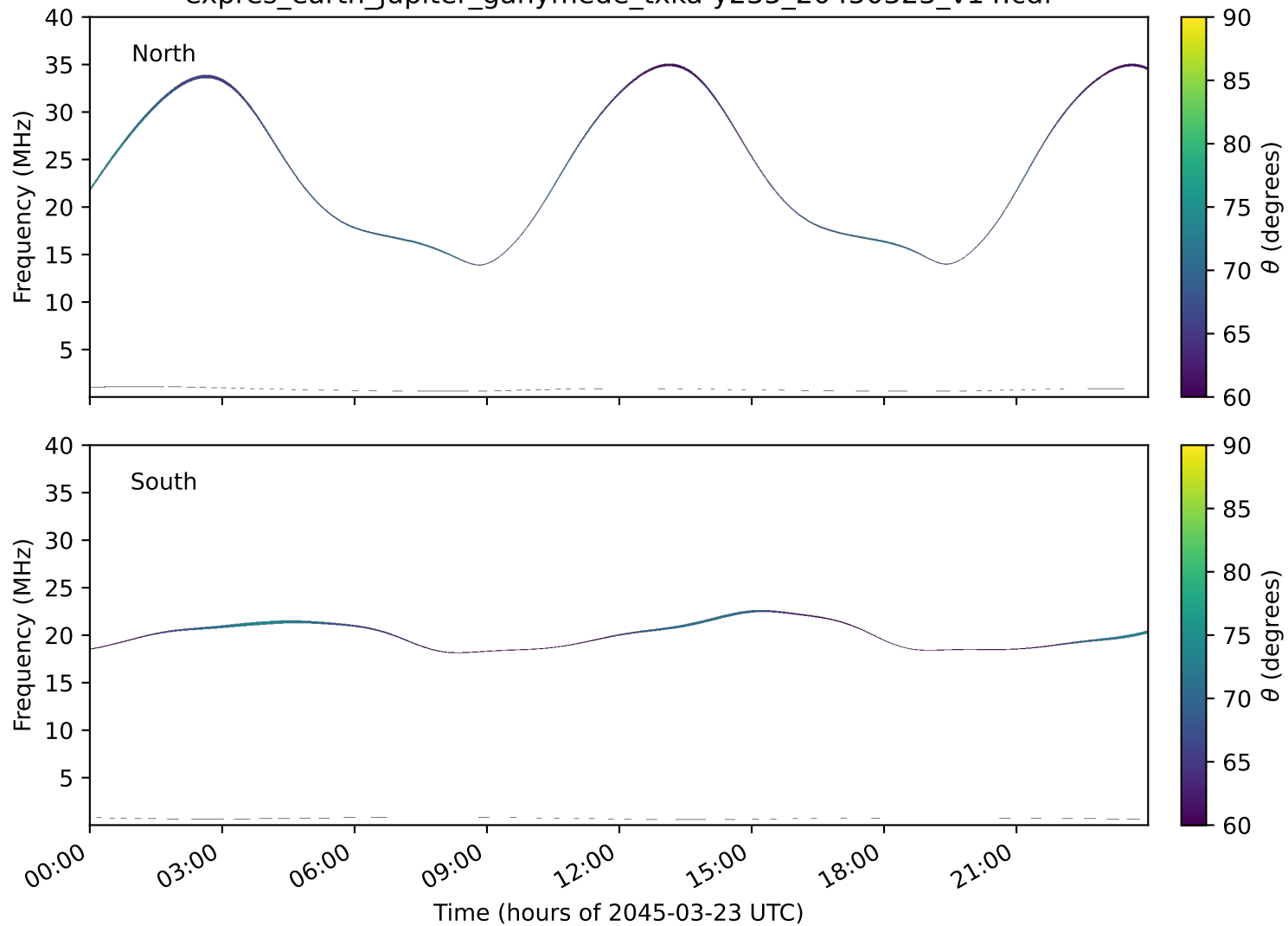
expres_earth_jupiter_ganymede_txka-y235_20450323_v14.cdf
