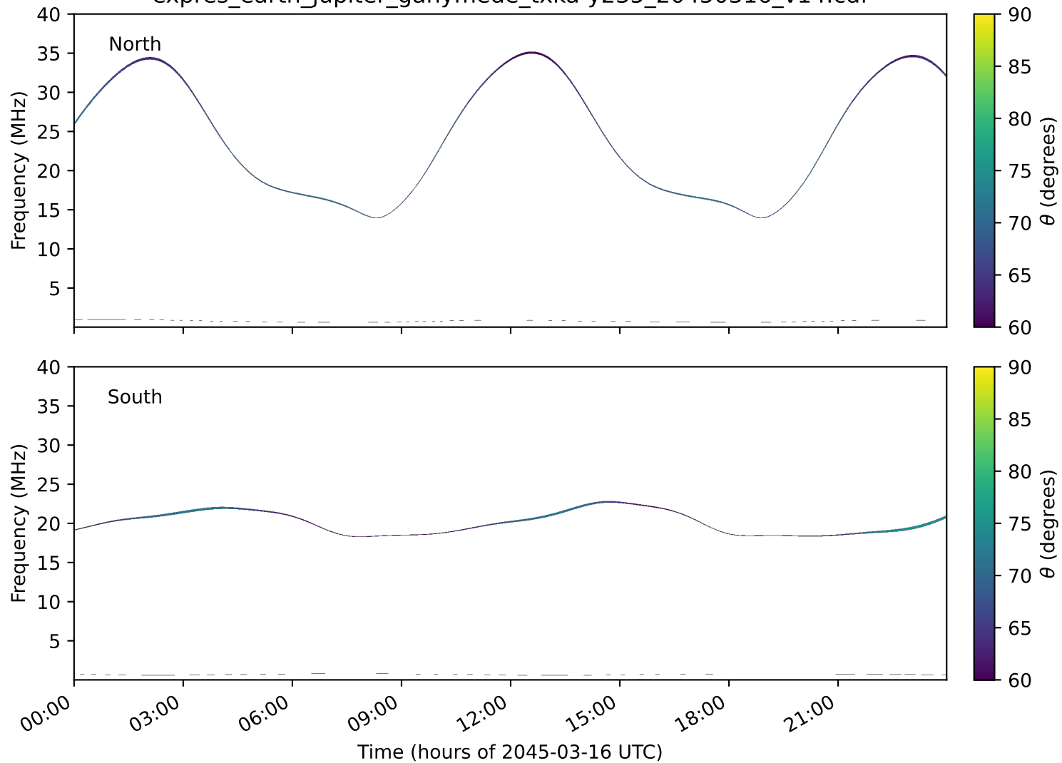
expres_earth_jupiter_ganymede_txka-y235_20450316_v14.cdf
