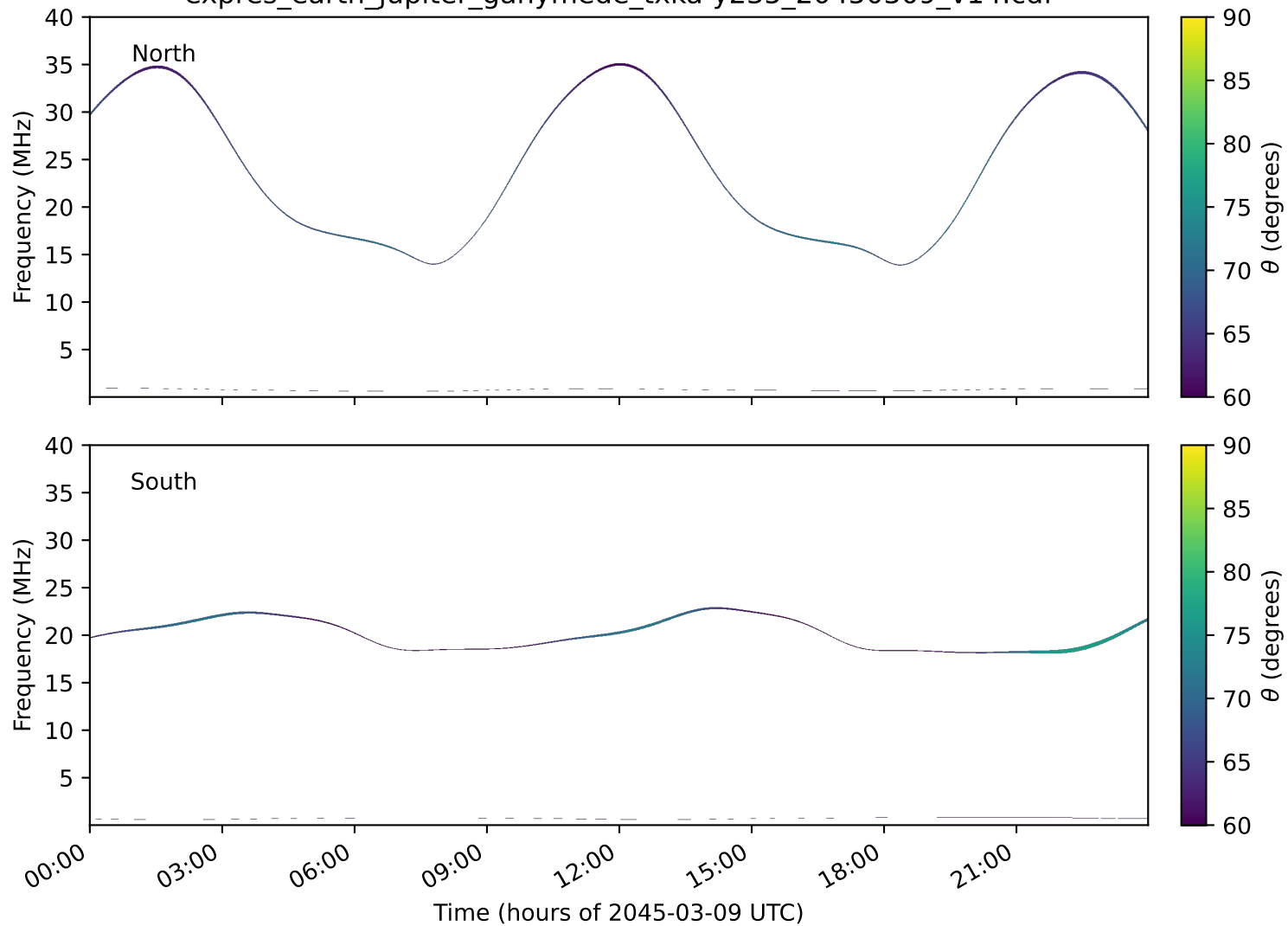
expres_earth_jupiter_ganymede_txka-y235_20450309_v14.cdf
