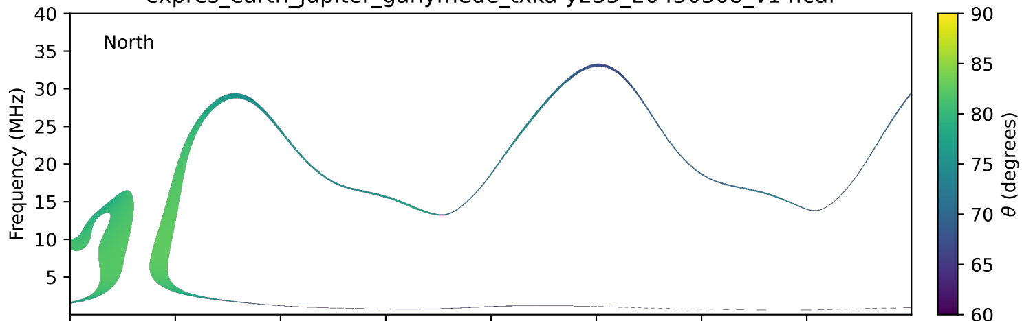
expres_earth_jupiter_ganymede_txka-y235_20450308_v14.cdf
