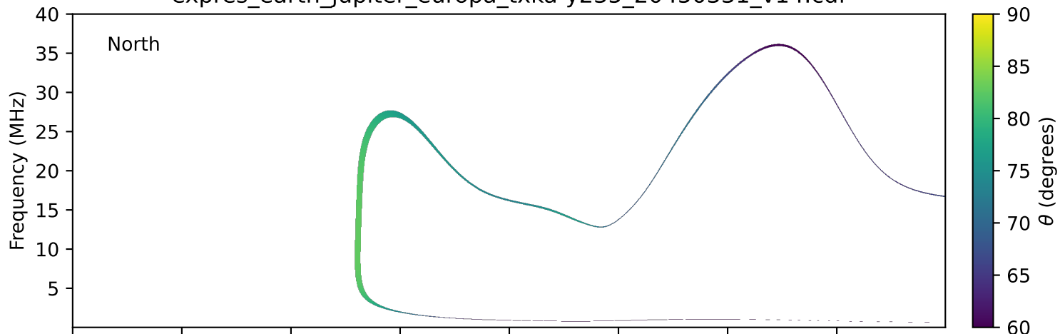
expres_earth_jupiter_europa_txka-y235_20450331_v14.cdf
