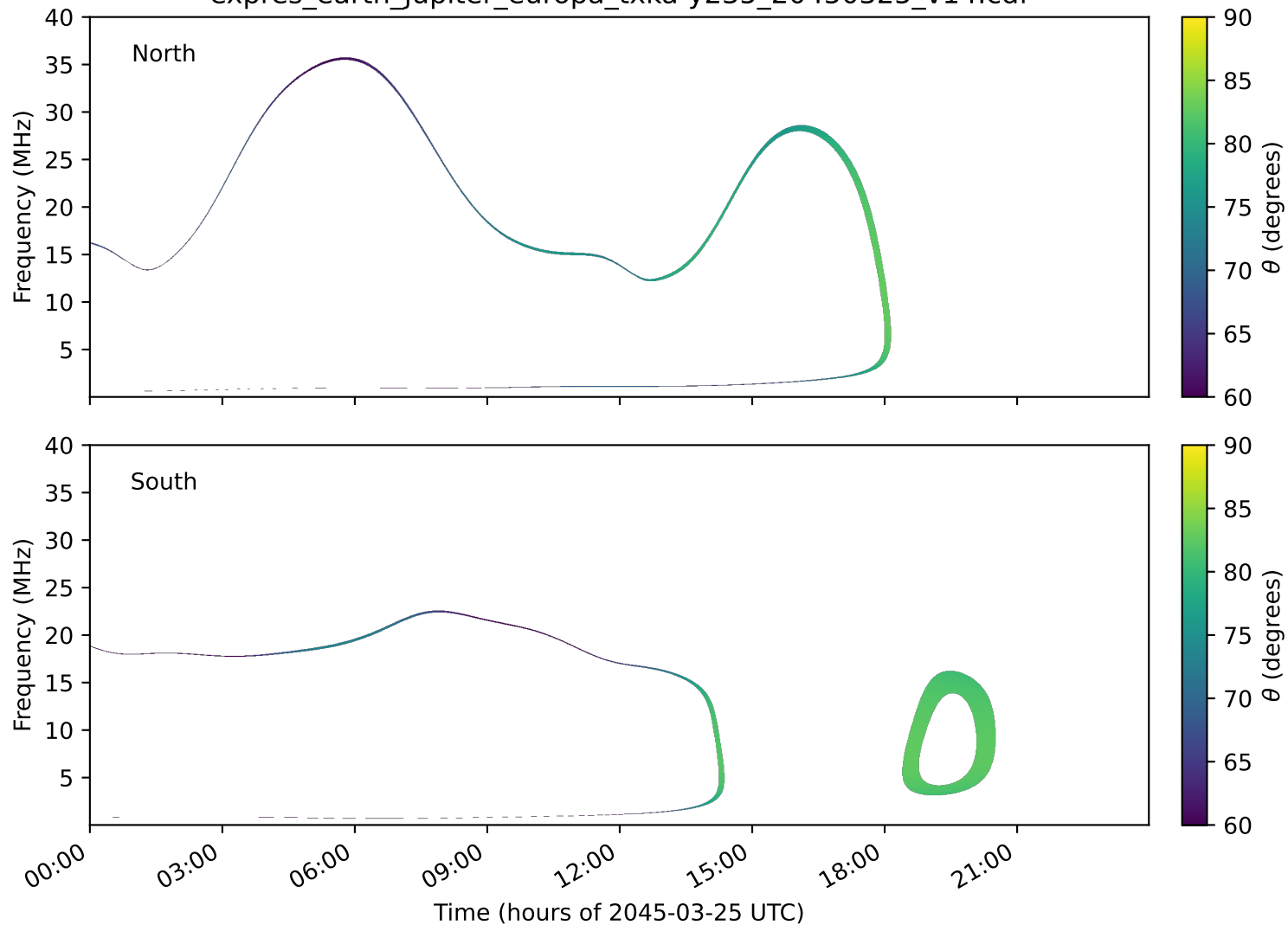
expres_earth_jupiter_europa_txka-y235_20450325_v14.cdf
