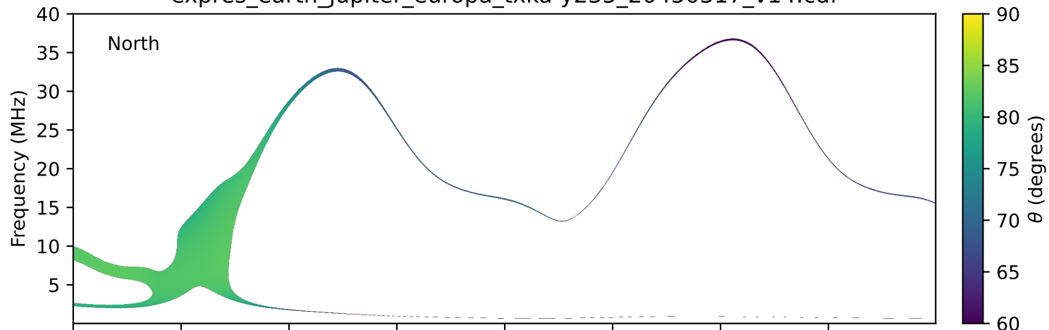
expres_earth_jupiter_europa_txka-y235_20450317_v14.cdf
