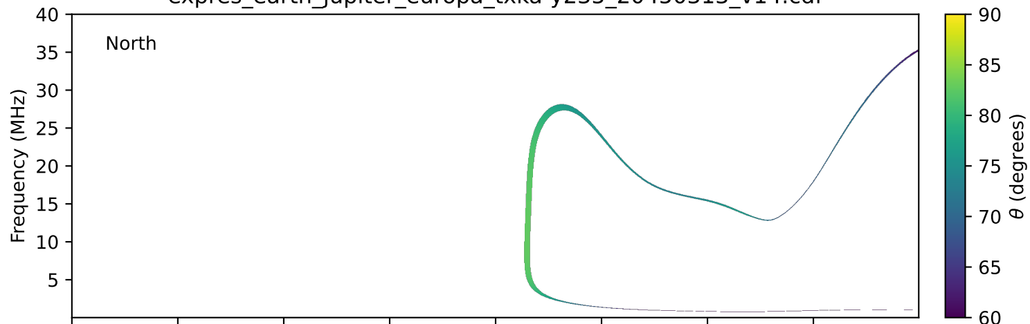
expres_earth_jupiter_europa_txka-y235_20450313_v14.cdf
