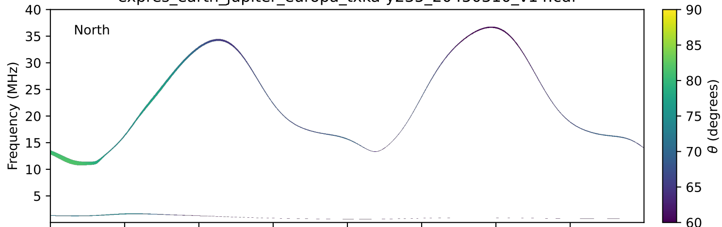
expres_earth_jupiter_europa_txka-y235_20450310_v14.cdf
