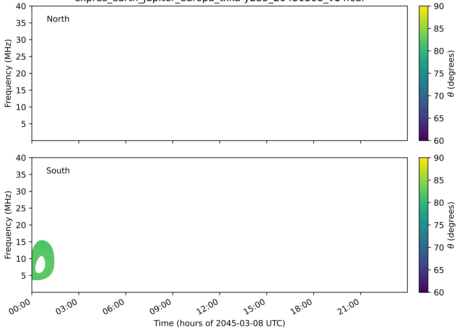
expres_earth_jupiter_europa_txka-y235_20450308_v14.cdf
