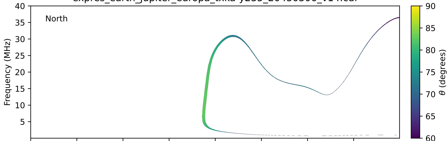
expres_earth_jupiter_europa_txka-y235_20450306_v14.cdf
