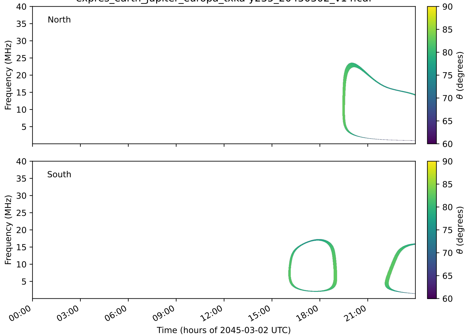
expres_earth_jupiter_europa_txka-y235_20450302_v14.cdf
