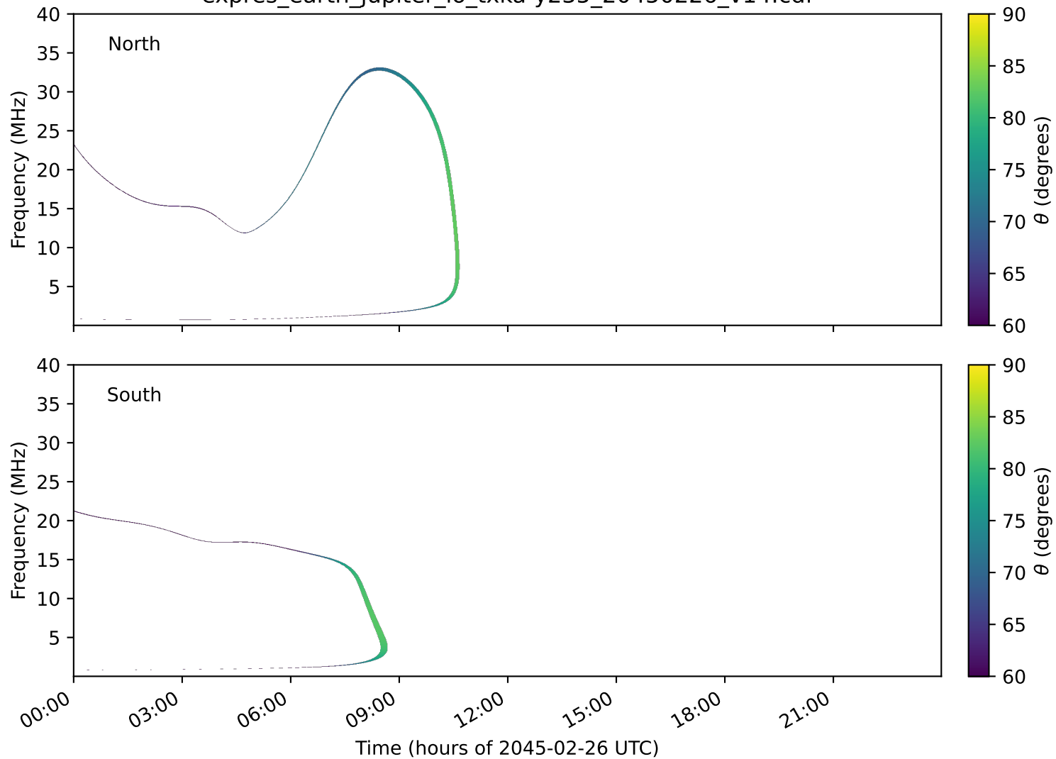
expres_earth_jupiter_io_txka-y235_20450226_v14.cdf
