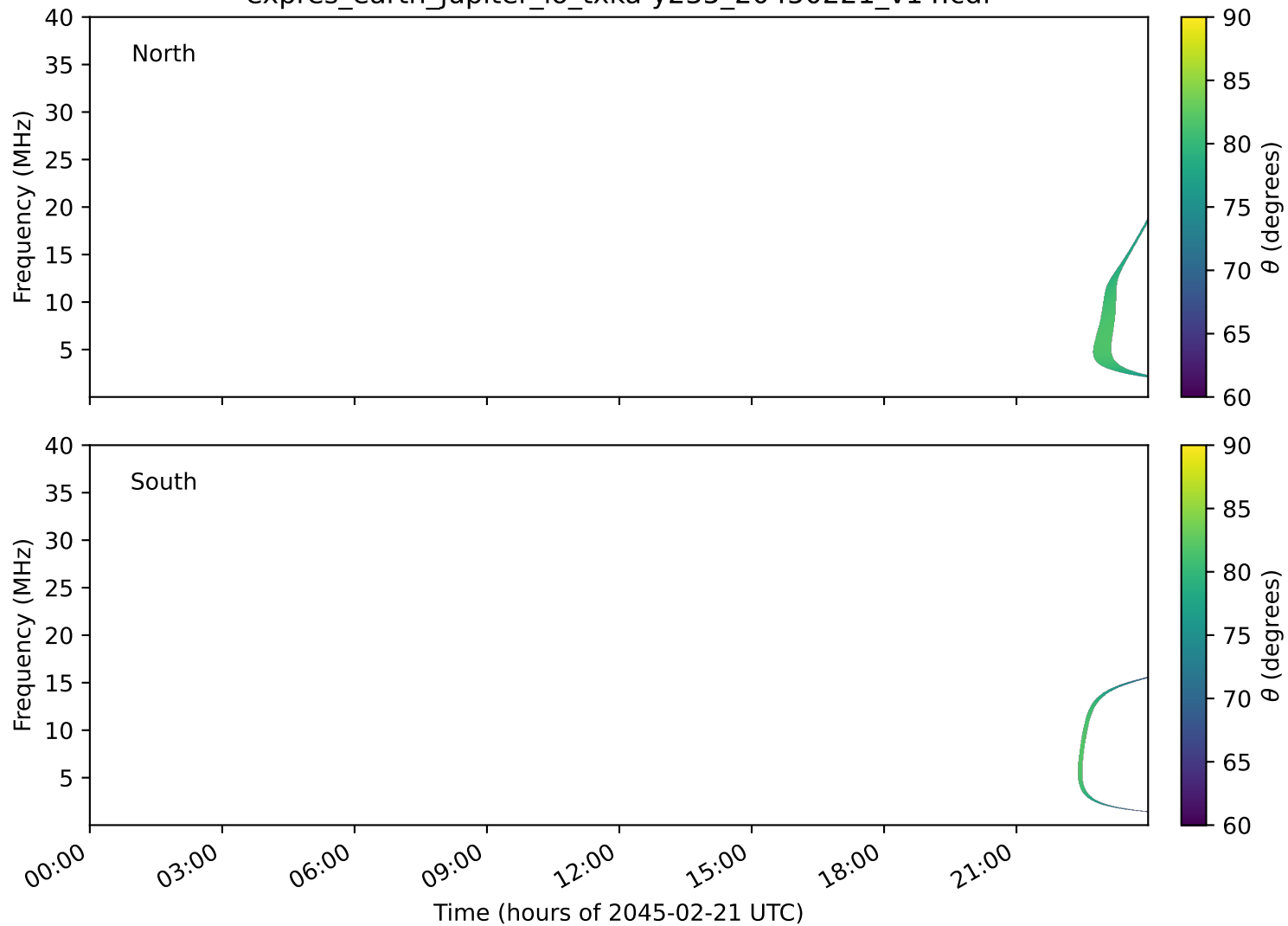
expres_earth_jupiter_io_txka-y235_20450221_v14.cdf
